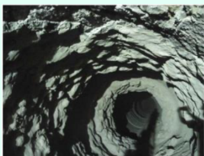
Coating and Buildup inside Cement Rotary Klin
