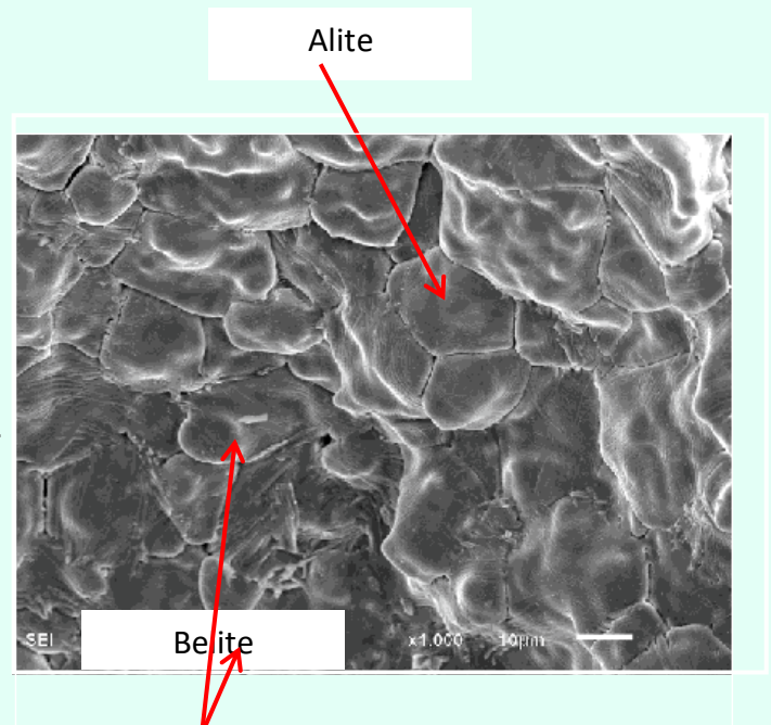
Scanning Electron-Micrograph of OPC Clinker
