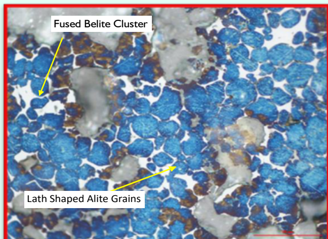
Optical Micrograph of control OPC clinker fired at 1450° C (50x)
