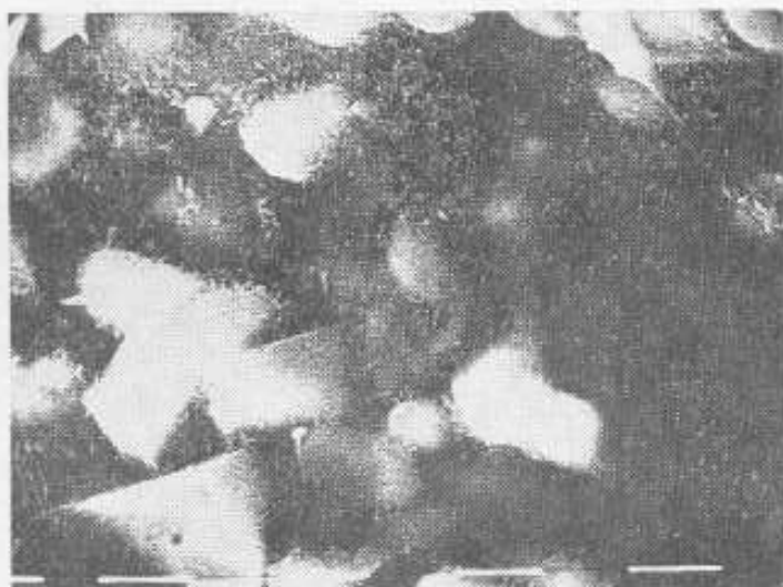
Plate II. Well developed alite and belite in yellow clinker
