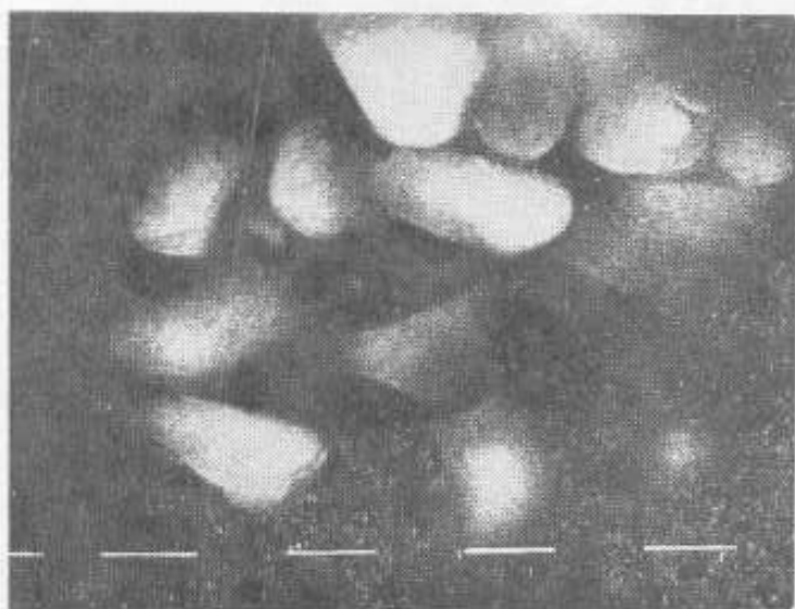
Plate III. Well developed alite and belite in brown clinker
