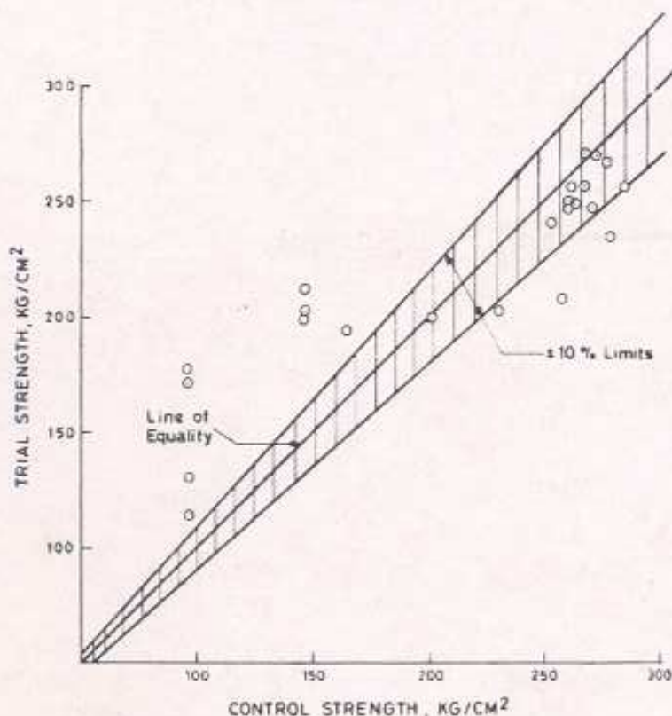
Fig 1 Comparison of 28-day Compressive Strength for Control and Trial Concretes-NCB Technology
