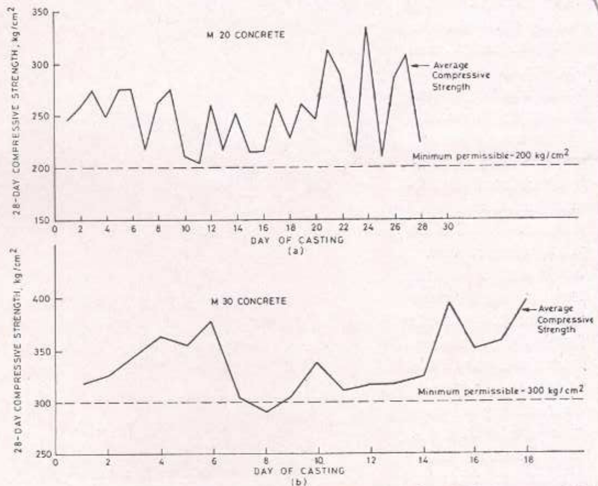
Fig 2 Quality Control Chart for (a) M 20 Concrete and (b) M 30 Concrete, Field (NCB Technology)
