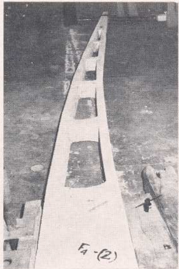
Fig 3 Typical pole under load test
